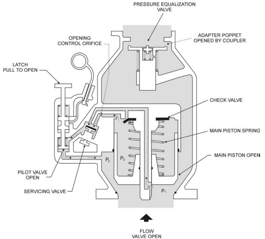
Figure A Valve Open
