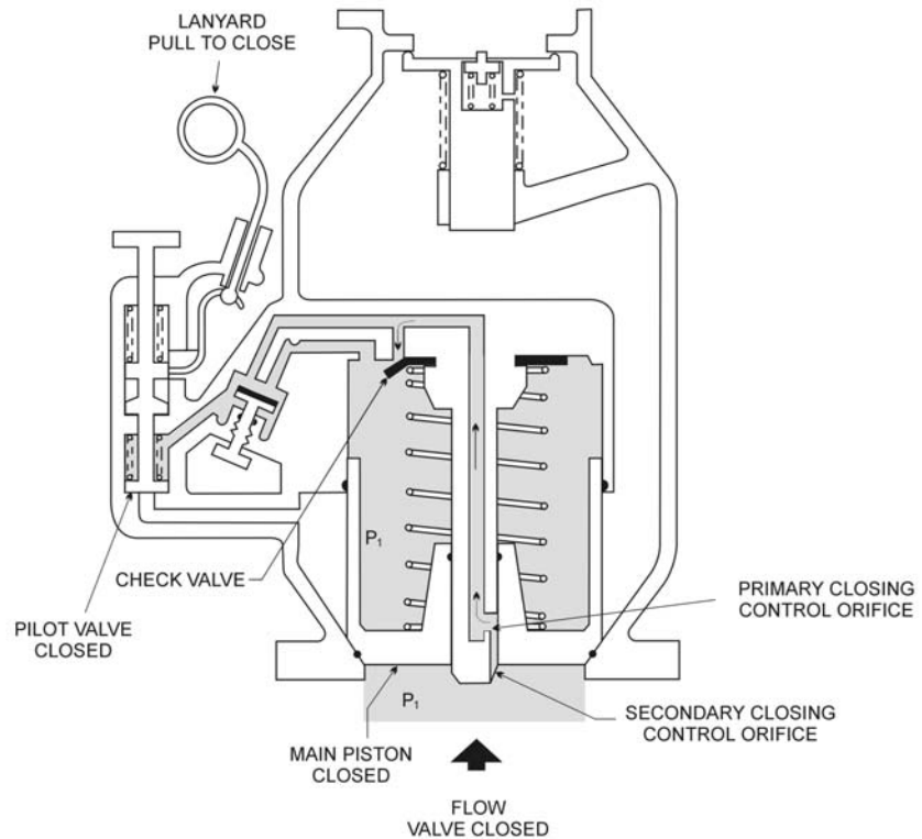
Figure B Valve Closed
