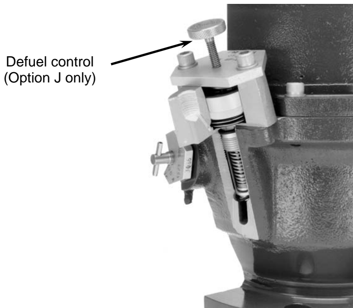
AIR OPERATED PILOT (with defuel capability)
