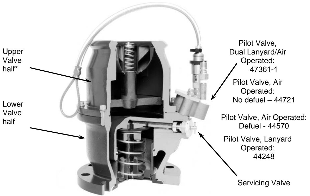
Typical Dual Air/Lanyard Operated Hydrant Valve
